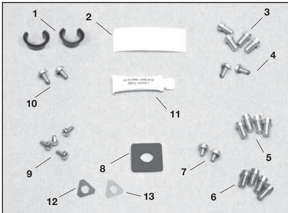
Figure 2 - Installation Kit Contents
